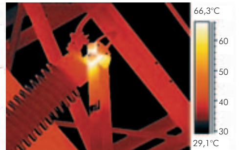
Find incorrectly secured connections
