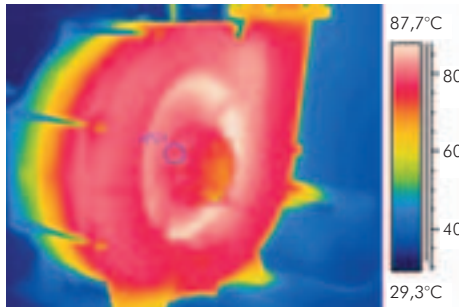
Overloaded pump
